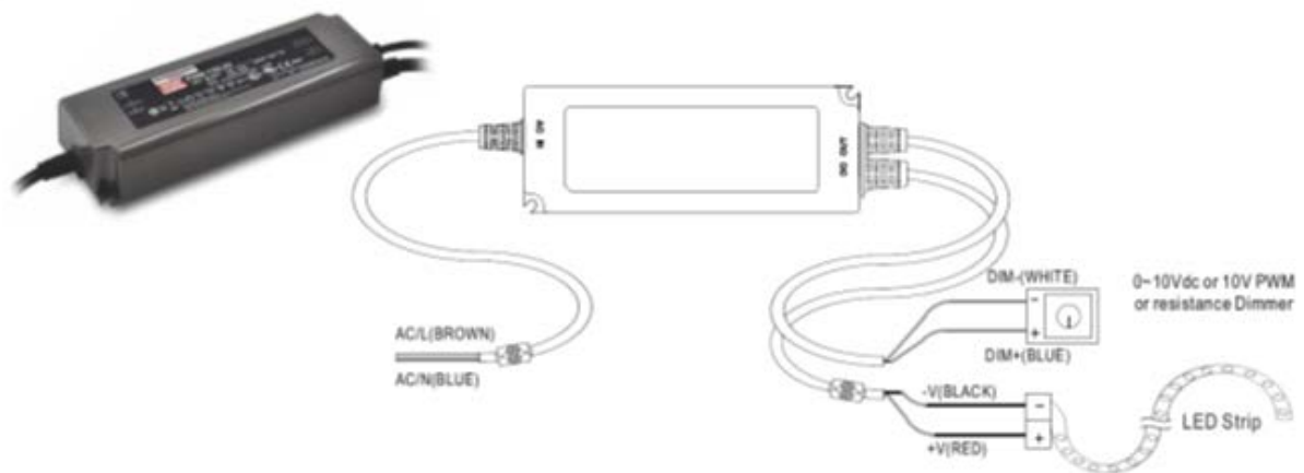
Figur 2-1: LED driver
