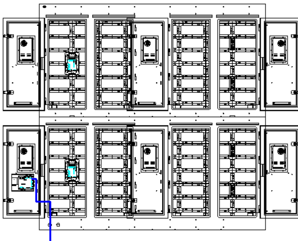
RJ45 signal input cable
