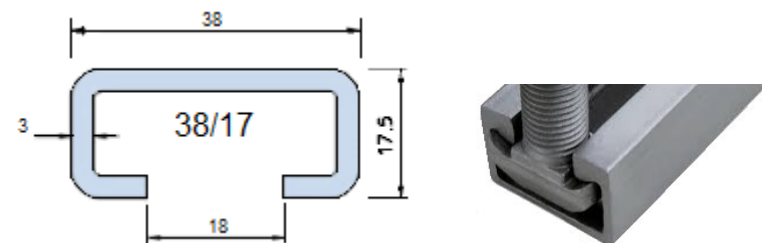
Figur 1: Halfen-skinne
