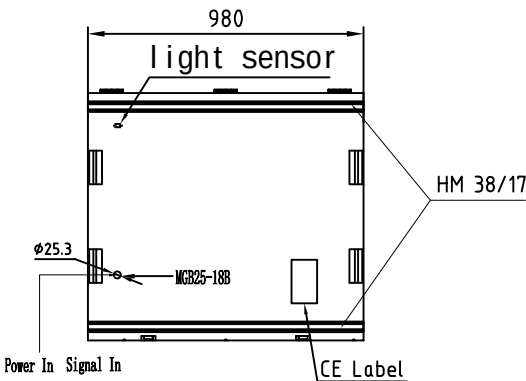
Back View
