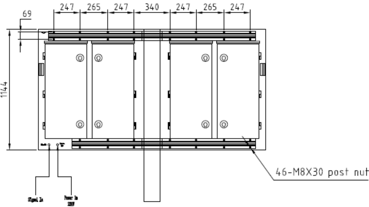
Left View
