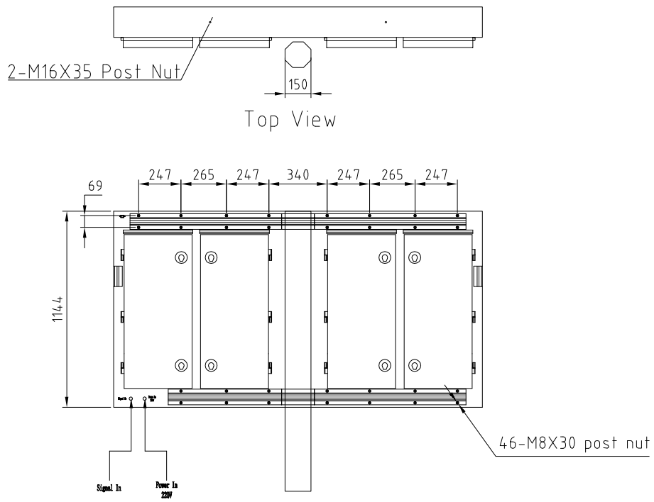
Back View
